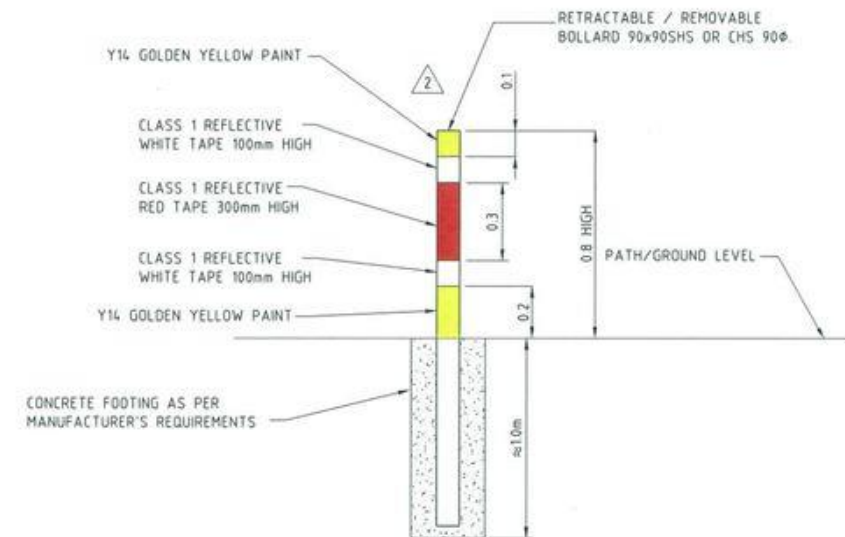
RETRACTABLE / REMOVABLE BOLLARD-SECTION DETAILS (REFER TO NOTE 10)
